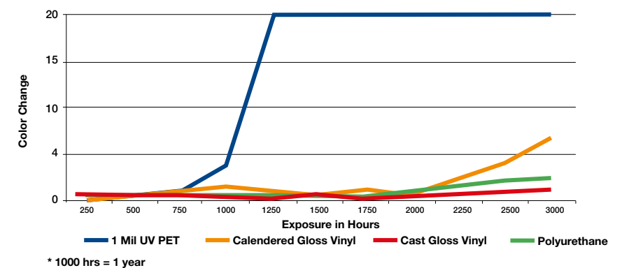
Xe Arc Testing UV Flexo Ink (Black) - PVC Base
