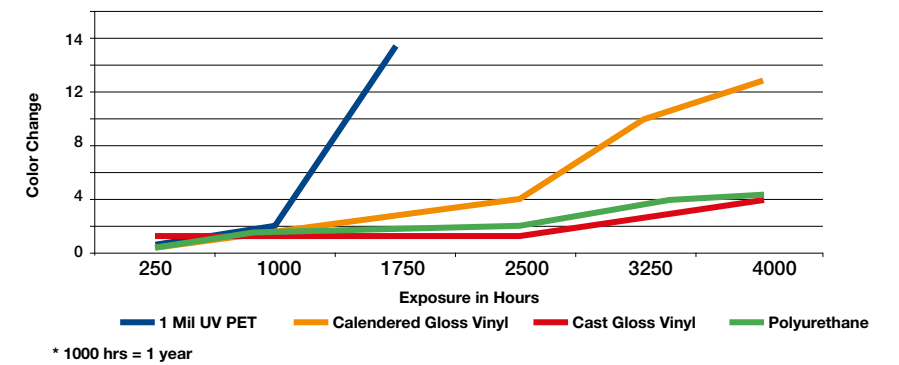
Xe Arc Testing with TT Ribbon (DNP R510HF) - PVC Base
